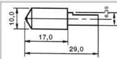
Rockwell 120° Wolpert Testor
