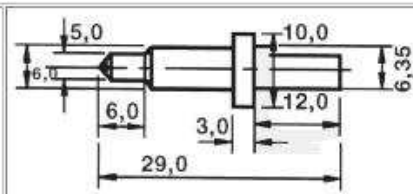
Rockwell 120° Testor Automat
